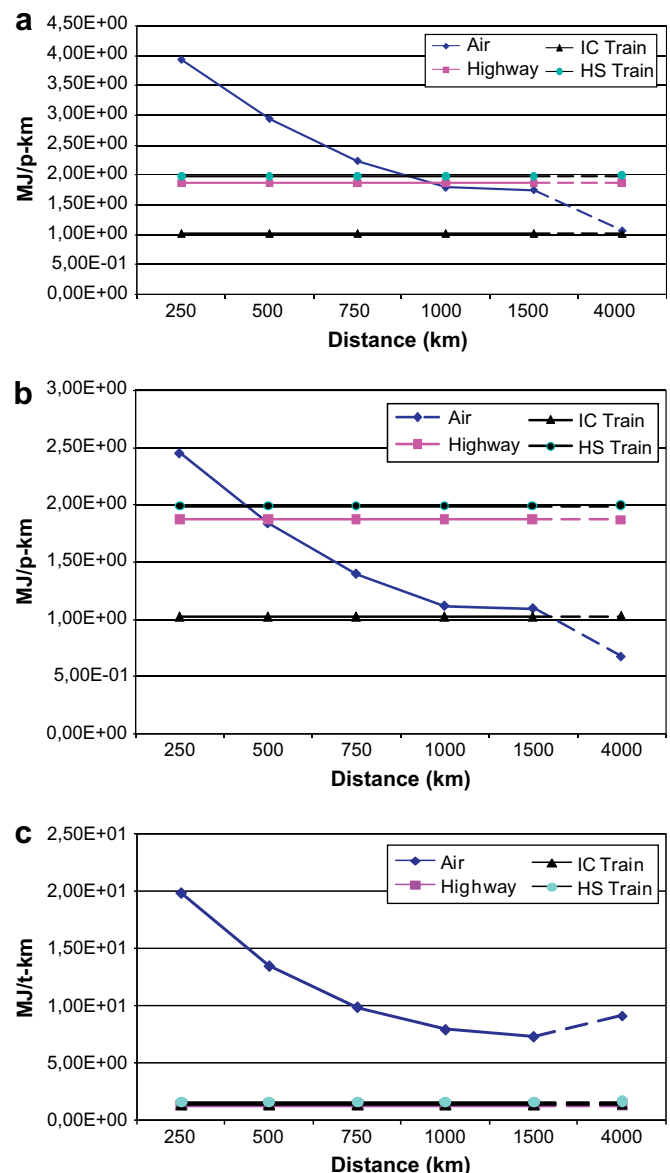
Fig. 2. (a) Comparison of embodied energy input per p-km for air, train and highway passenger transport. A 50% of maximum payload capacity was assumed for air transport. Air transport becomes competitive with High Speed train and highway car transport at a distance of 1000 km, while it is never competitive with intercity train. (b) Comparison of embodied energy input per p-km for air, train and highway passenger transport. An 80% of maximum payload capacity was assumed for air transport. Air transport becomes competitive with high speed train and highway car transport at a distance of 500 km, while it is never competitive with intercity train. (c) Comparison of embodied energy input per p-km for air, train and highway freight transport. Because of their small freight payload capacity, airplane performances are always much worse than all other modalities.
