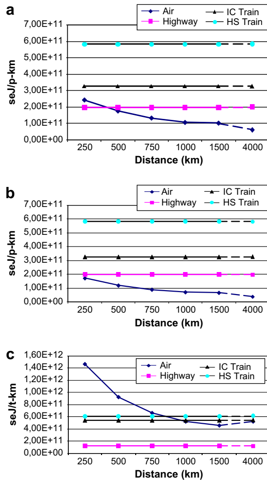
Fig. 3. (a) Comparison of energy input per p-km for air, train and highway passenger transport. An 80% of maximum payload capacity was assumed for air transport. Because of the marginal role of infrastructures for air transportation modalities and the increased importance of material infrastructures of the other modalities according to the Energy Synthesis method, air transport is always the most competitive transportation pattern, as far as energy is concerned. (b) Comparison of energy input per p-km for air, train and highway passenger transport. A 50% of maximum payload capacity was assumed for air transport. Under such an assumption, air transport becomes competitive with highway car transportation only for distances higher than 400 km. (c) Comparison of energy input per t-km for air, train and highway freight transport. Under an energy point of view, the most competitive transportation pattern is the highway truck modality.
