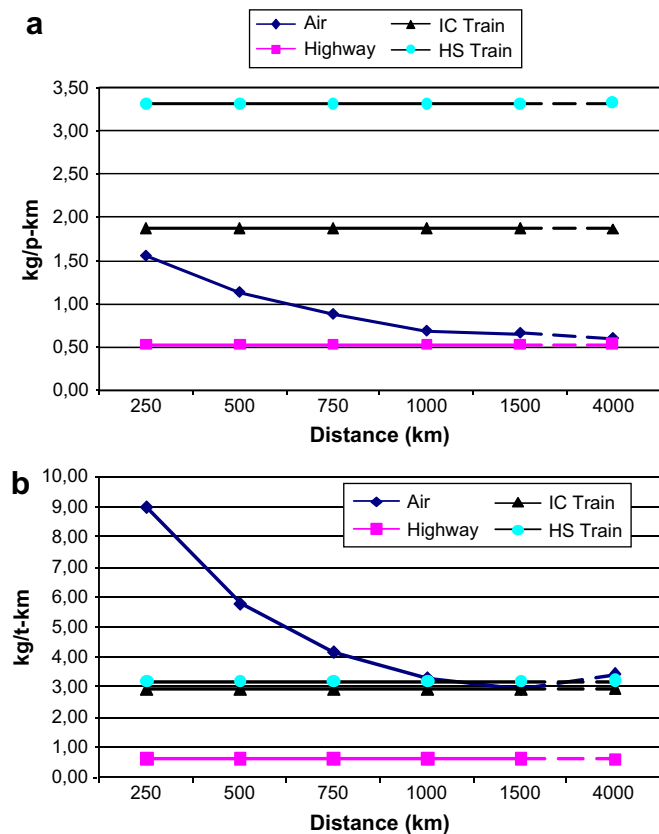
Fig. 1. (a) Comparison of material input per p-km for air, train and highway passenger transport. Air related MI (calculated under the assumption of 50% of maximum payload capacity) declines steadily with distance, due to the declining importance of infrastructure in such a transportation modality. Airplanes are always competitive with HS train and IC trains, concerning material intensity indicators, due to the dominating influence of infrastructure. (b) Comparison of material input per t-km for air, train and highway freight transport. Air related MI declines steadily with distance, due to the declining importance of infrastructure in such a transportation modality. Under the same assumptions used for (a), air transport is never competitive, while highway truck transport is always the less intensive option, as far as material intensity is concerned.
